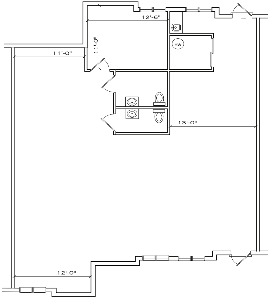
SUITE 562 1,630 SQ. FT.
